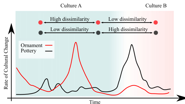
Fig. 5. Inferred relationship between the population structure as defined by pottery style and the inter-site dissimilarity in pottery and personal ornament.
